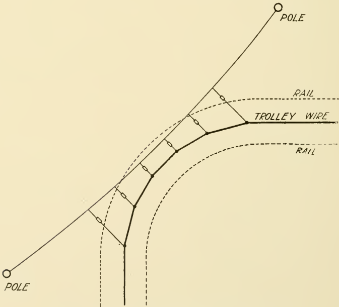
Fig. 193. Simple Curve Suspension Using Two Poles
